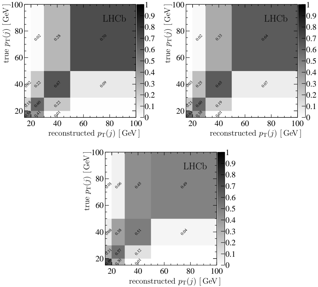
Figure 5. Detector-response matrices for (left) D^0 -, (right) D^+ - and (bottom) DV-tagged charm jets. The shading represents the interval-to-interval migration probabilities ranging from (white) 0 to (black) 1 such that each row sums to unity when the underflow and overflow bins are included. Jets with true (reconstructed) p_T(j) in the 20–100 GeV region but whose reconstructed (true) p_T(j) is either below 15 GeV or above 100 GeV are included in the unfolding but not shown graphically.
