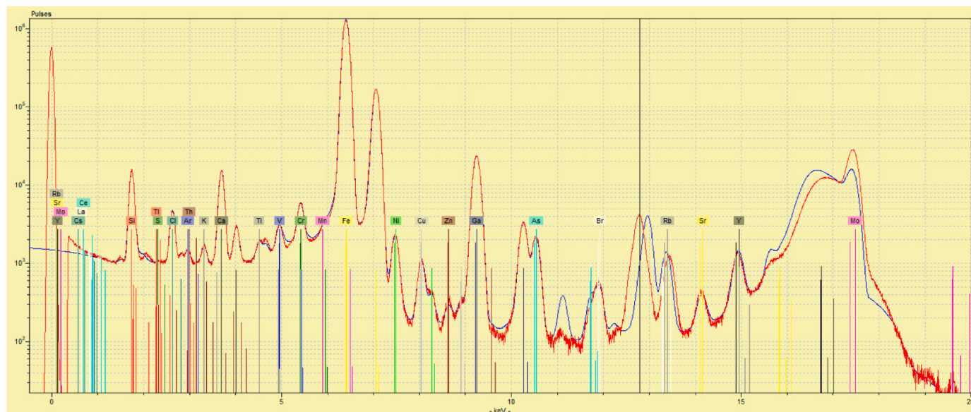
Fig. 2. An example of the whole spectra of a soil sample analyzed by Picofox S2.
