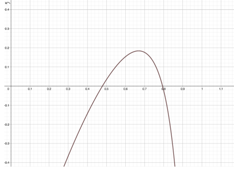
Figure 4.1: The plot of G^\tau for \alpha = 1 .
