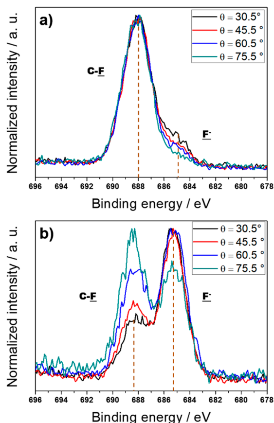
Figure 5. F1s XP-high resolution regions of ZnO-CF x nanocomposites having an inorganic phase volume fraction of \phi = 0.15 as a function of \theta and subject to thermal treatment in an oxygenated atmosphere (a) or deposited with an auxiliary O 2 flow (b).
