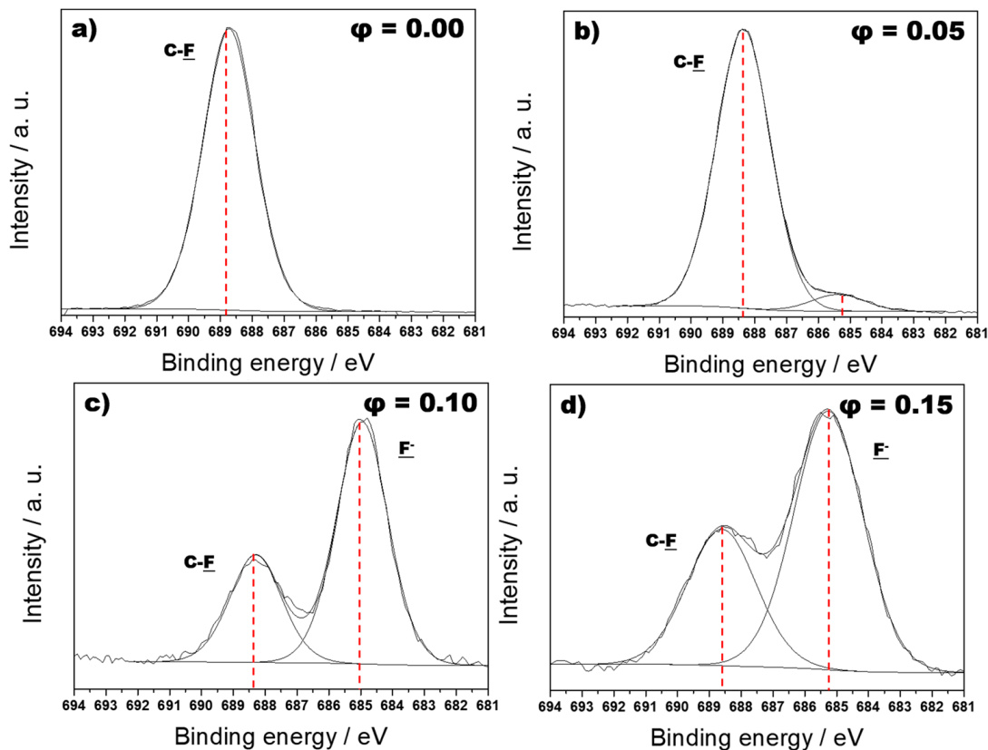
Figure 3. F1s XP-high resolution regions of ZnO-CF x nanocomposites having an inorganic phase volume fraction \phi = 0 (a), \phi = 0.05 (b), \phi = 0.10 (c), and \phi = 0.15 (d).
