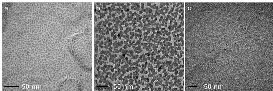
Figure 1. Transmission electron microscopy (TEM) micrographs of ZnO-CF x nanocomposites having an inorganic phase volume fraction of \phi = 0.05 (a); \phi = 0.10 (b); and \phi = 0.15 (c).
