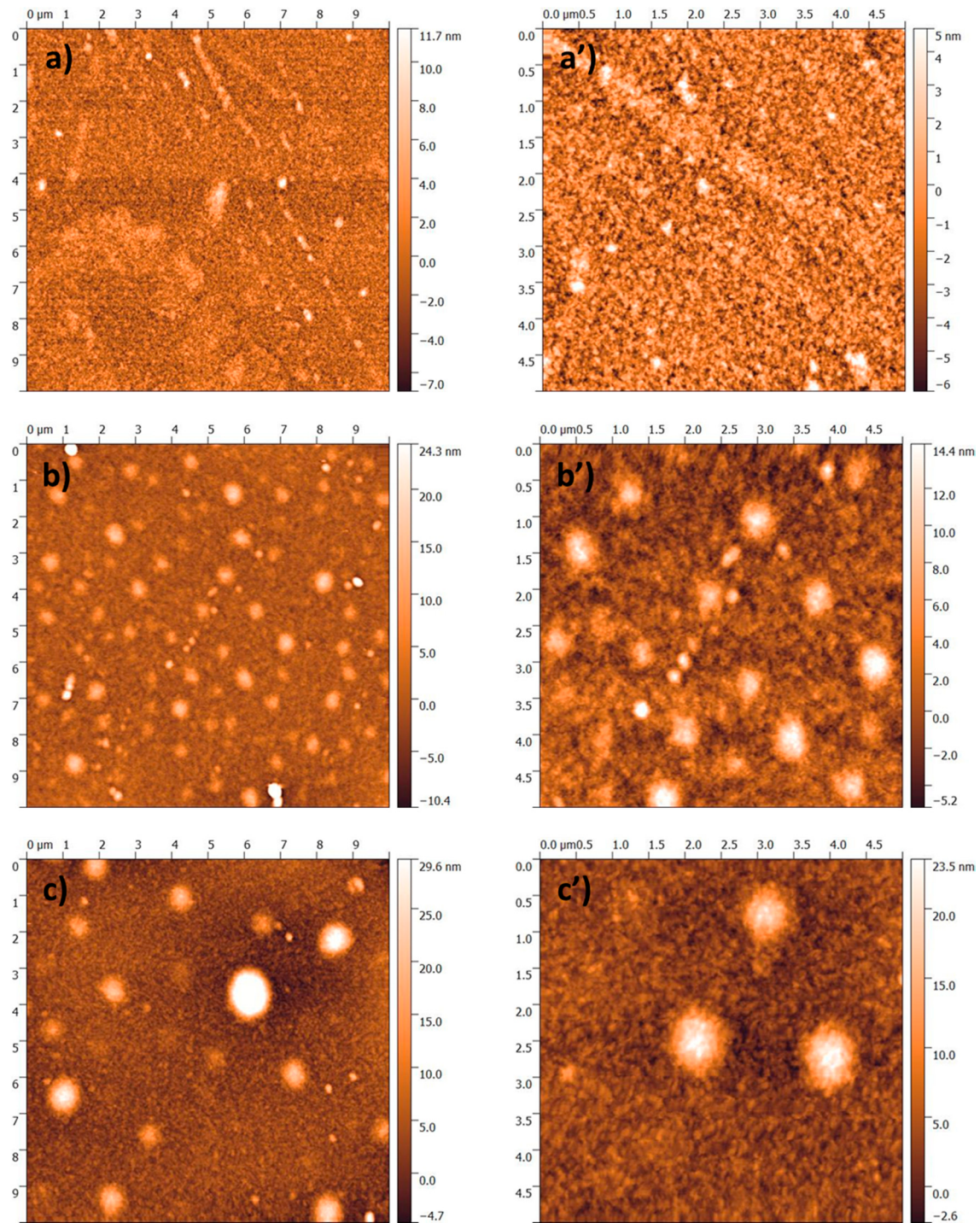
Figure 2. Atomic force microscopy (AFM) micrographs of ZnO-CF x nanocomposites having an inorganic phase volume fraction of \phi = 0.05 (a–a'), \phi = 0.10 (b–b'), and \phi = 0.15 (c–c').
