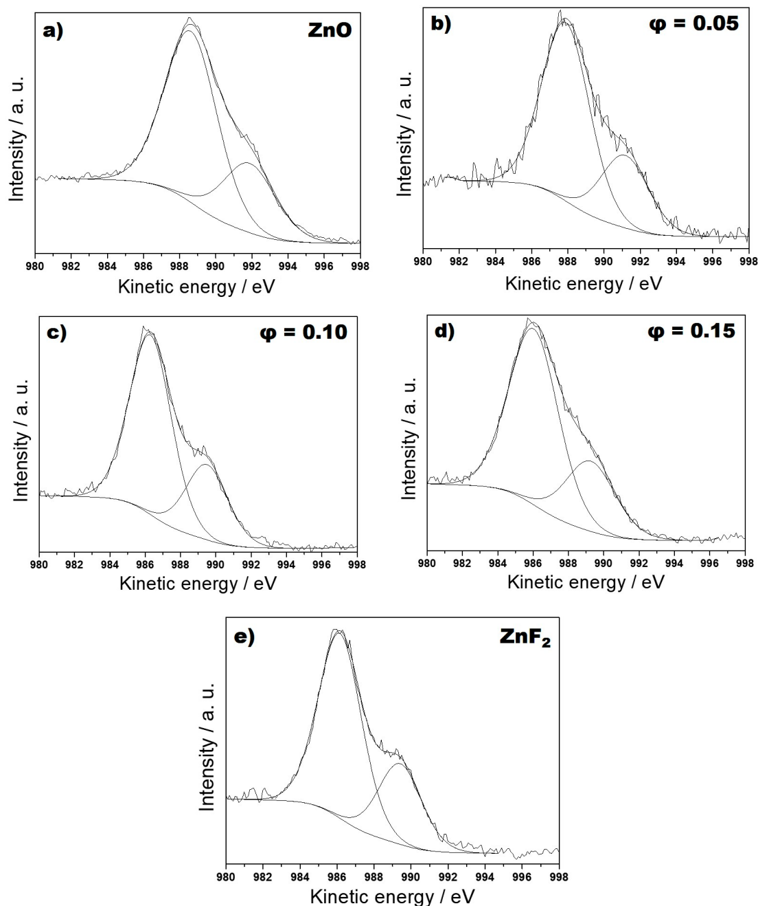
Figure 4. \text{ZnL}_3\text{M}_{45}\text{M}_{45} XP-high resolution regions of \text{ZnO-CF}_x nanocomposites having an inorganic phase volume fraction of \phi = 0.05 (b); \phi = 0.10 (c); and \phi = 0.15 (d). The same region for a pure ZnO film (a) and a \text{ZnF}_2 standard (e) is also reported, for comparison.
