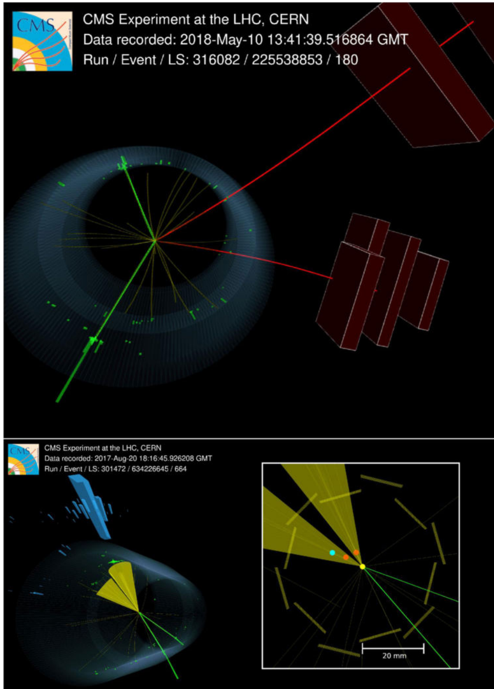
Extended Data Fig. 2 | Higgs boson candidate events. (upper) An event display of a candidate H \rightarrow ZZ \rightarrow e\mu\mu . (lower) An event display of an H \rightarrow bb candidate produced in association with a boson decaying into an electron-positron pair, in pp collisions at \sqrt{s} = 13 TeV recorded by CMS. The charged-particle tracks, as reconstructed in the inner tracker, are shown in yellow; the electrons are shown in green, the energy deposited by the electrons in the ECAL is shown as large green towers, the size of which is proportional of the amount
