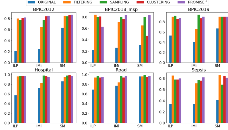
Figure 6: Fmeasure of precision and fitness: PROMISE + vs related methods ( ORIGINAL , FILTERING , SAMPLING and CLUSTERING ) by varying the process discovery algorithm among Hybrid ILP Miner (ILP), Inductive Miner (IMi) and Split Miner (SM).
