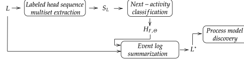
Figure 3: Schema of the PROMISE + method.
