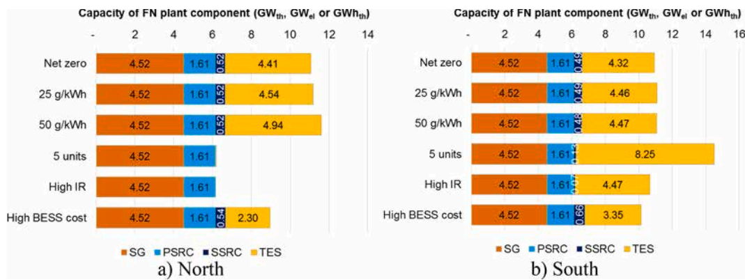
Fig. 5. Cost-optimal configurations of flexible nuclear plants across various scenarios for North and South systems. SG and PSRC sizes are kept constant for all scenarios and SSRC and TES sizes are optimised.
