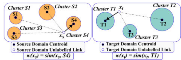
Fig. 3. Stage II—weighting of unlabeled links
