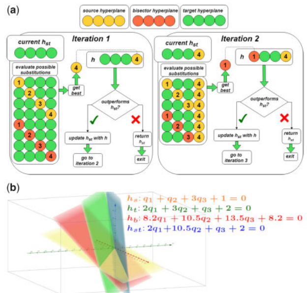
Fig. 5. (a) An example of two consecutive iterations of the identification of the best substitution on the current hyperplane (function get\_best\_sub in Algorithm 1–Line 19). (b) A graphical representation of the combination of source (yellow), target (green) and bisector (red) hyperplanes. The method returns the new combined hyperplane (blue). (Color version of this figure is available at Bioinformatics online.)
