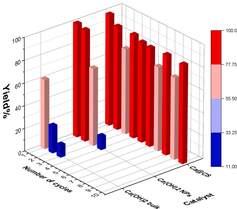
Fig. 8. Comparison among commercial Ca(OH) 2 , unsupported submicrometric particles (Ca(OH) 2 NPs), and Ca@CS catalysts in recyclability tests.
