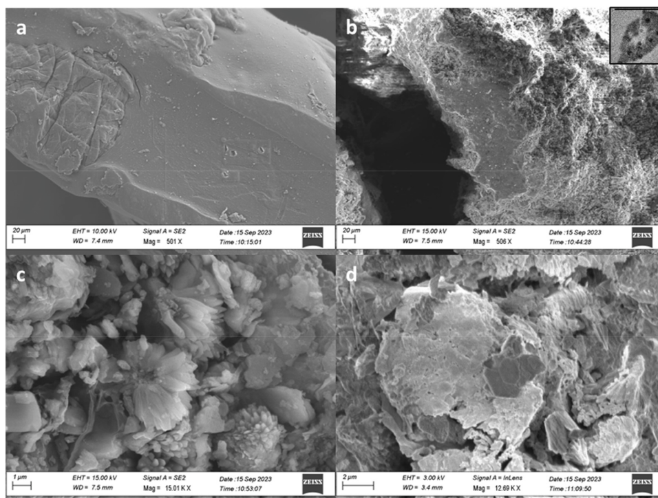
Fig. 4. FESEM images of CS (a) and Ca@CS catalyst (b-d) samples. A TEM image in the inset b shows a chitosan flake with nanometric structures on it (scale bar: 1 µm).
