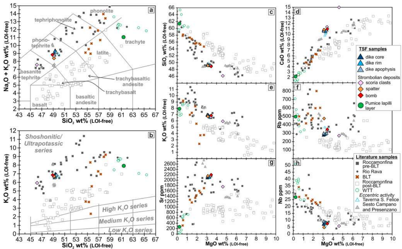
Figure 8. (a and b) Total Alkali versus Silica (TAS; Le Bas et al., 1986) and K_2O versus SiO_2 (Le Maitre et al., 2002), and (c–h) selected major oxides and trace elements versus MgO diagrams for the investigated samples from the Taverna San Felice (TSF) magmatic dike (dike core, dike margin, apophysis) and TSF Strombolian deposits and pumice lapilli layer. Literature samples for the Roccamonfina volcano (Beccaluva et al., 1991; Carter et al., 1978; Conticelli et al., 2002, 2007, 2009; D'Antonio et al., 1996; Di Girolamo, 1968; Giannetti, 1996, 2002; Giannetti & Ellam, 1994; Giannetti & Luhr, 1983; Hawkesworth & Vollmer, 1979; Luhr & Giannetti, 1987; Martelli et al., 2004; Rouchon et al., 2008; Santello, 2010; Vollmer, 1976; Vollmer & Hawkesworth, 1980), and for the peripheral vents of TSF, Sesto Campano and Presenzano, to the NE of the volcano edifice (Di Girolamo et al., 1991) are also reported for comparison.
