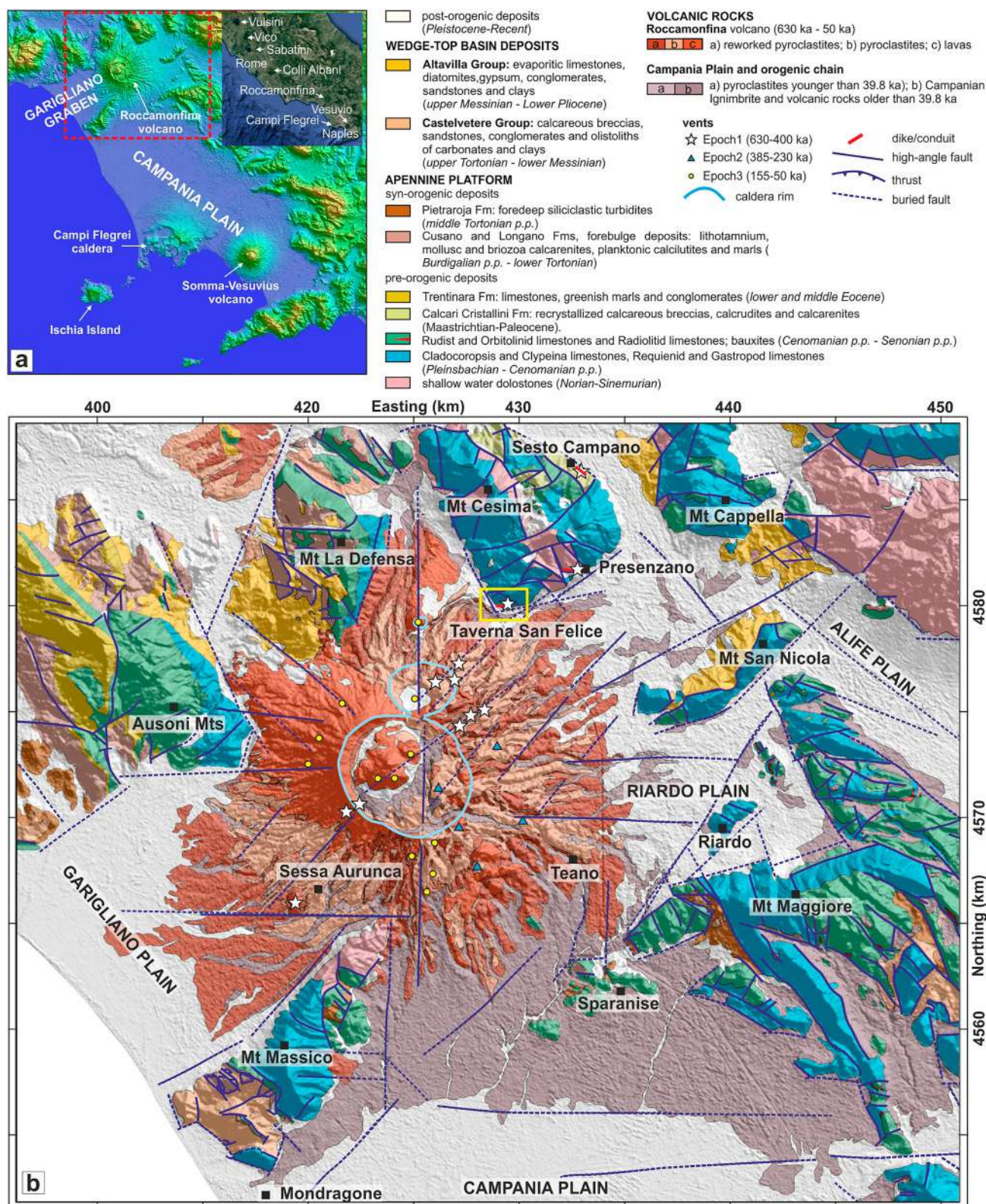
Figure 1. (a) Digital Elevation Model (DEM) of the Campania Plain-Garigliano Graben area extracted from ALOS3D DEM (Japan Aerospace Exploration Agency, 2021), with the inset at the upper right highlighting the volcanic districts of the Roman and Campanian magmatic provinces of central-southern Italy and the red dashed rectangle showing the position of panel (b). (b) Geological map of the Garigliano Graben (modified after Vitale & Ciarcia, 2018), the yellow box indicates the study area.
