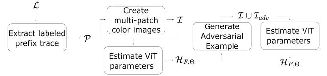
Fig. 1. JARVIS pipeline.
