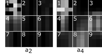
Fig. 10. Maps of attention of two prefix traces of BPI13P, which are correctly labeled with “a2” (“Accepted-In Progress”) and “a4” (“Completed-Closed”), respectively. The maps are shown in the luminosity channel of the LAB space. The numbers identify the names of the views in the event log: 1-“activity”, 2-“resource”, 3-“timestamp”, 4-“impact”, 5-“org country”, 6-“org group”, 7-“org role”, 8-“product”, 9-“resource country”.
