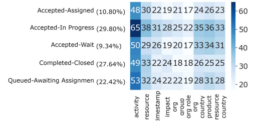
Fig. 13. Heatmap of the global patch lightness computed activity by activity (axis Y) for all the views in the event log BPI13P. For each (next) activity category, the support of the category is reported in the brackets.
