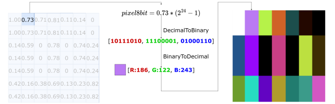
Fig. 4. Conversion of the Word2Vec embedding representation shown in Fig. 3 into an imagery color patch.
