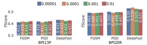
Fig. 9. Macro FScore measured in BPI13P and BPI20R by varying the \epsilon among 0.01, 0.001 (default), 0.0001 and 0.00001 with FGSM, PGD and DeepFool.
