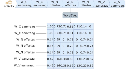
Fig. 3. Word2Vec embedding of the sequence of activities enclosed in the sample prefix trace shown in Fig. 2.
