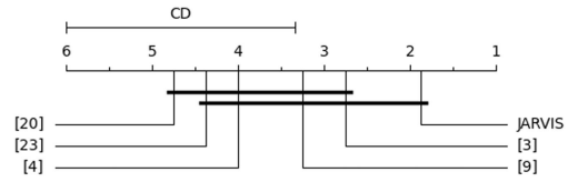
Fig. 8. Comparison of FScore of JARVIS and the state-of-the-art methods defined in [3], [4], [9], [20] and [23] with the Nemenyi test. Groups of approaches that are not significantly different (at p \leq 0.05 ) are connected.
