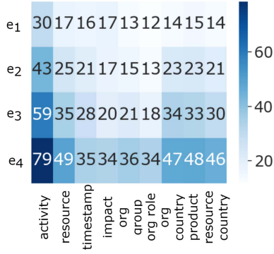
Fig. 14. Heatmap of the global intra-patch event lightness computed for each event position (axis Y) in the prefix traces the event log BPI13P for each event log view (axis X).
