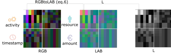
Fig. 7. Map of attention produced in the RGB space (left side) for the prediction of the next-activity of the imagery representation shown in Fig. 5 of the sample prefix trace reported in Fig. 2. Transformation of the map of attention from the RGB space to the LAB space (central side). Luminosity (L) channel of the map of attention produced in the LAB space (right side).
