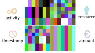
Fig. 5. Multi-patch color image with size 14 \times 14 \times 3 . This image is obtained by distributing the four image patches of size 7 \times 7 \times 3 , produced for the views “activity”, “resource”, “timestamp” and “amount” of the prefix trace shown in Fig. 2, into a 2 \times 2 patch grid.
