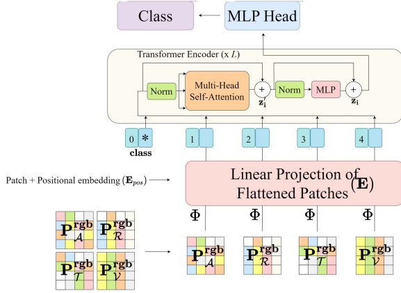
Fig. 6. ViT architecture.
