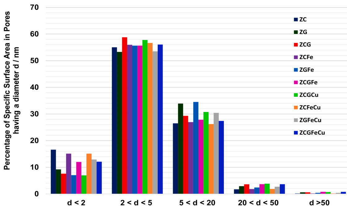
Fig. 2. Porosity Distribution: Percentage of Specific Surface Area in pores having a diameter d / nm.
