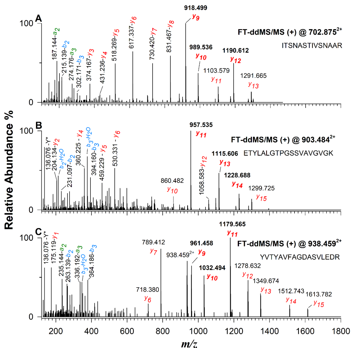
Figure 2. High-resolution HCD-MS/MS spectra of marker peptides of the spirulina allergenic protein P72508 (C-phycocyanin beta subunit): (A) ITSNASTIVSNAAR at m/z 702.875 2+ , (B) ETYLALGTPGSSVAVGVGK at m/z 903.484 2+ , and (C) YVTYAVFAGDASVLEDR at m/z 938.459 2+ . Major y-type product ions, useful for multiple ion monitoring (MRM) acquisitions, are labeled in bold.
