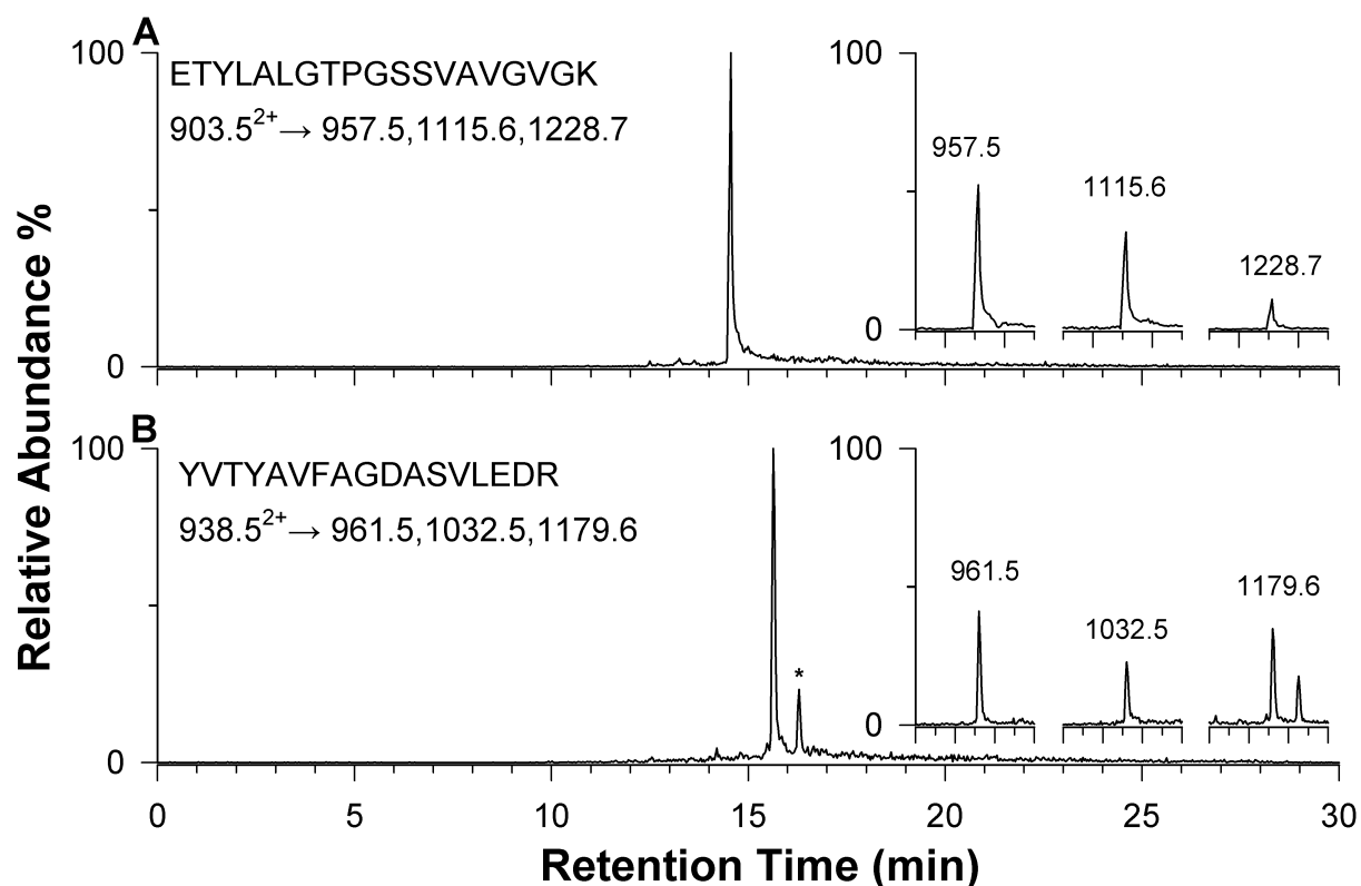
Figure 3. Chromatograms by RPLC-ESI-LIT-MS/MS in multiple reaction monitoring (MRM) of marker peptides of the spirulina allergenic protein C-phycocyanin beta subunit in spiked cookies at 2.5 mg TotProt/gmatrix : (A) ETYLALGTPGSSVAVGVGK at m/z 903.5 2+ , and (B) YVTYAVFAGDASVLEDR at m/z 938.5 2+ . Major y -type product ions detected in CID-MS/MS spectra were used to extract the ion currents (see bold product ions in Figure 2 ). Insets show the individual measured transitions.
