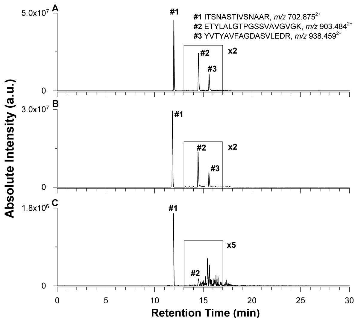
Figure 1. XIC chromatograms by RPLC-ESI-FTMS in positive ion mode of the marker peptides of C-phycocyanin beta subunit (P72508) ITSNASTIVSNAAR at m/z 702.875 2+ (#1), ETYLALGTPGSSVAVGVGK at m/z 903.484 2+ (#2), and YVTYAVFAGDASVLEDR at m/z 938.459 2+ (#3) occurring in spirulina powder samples (A), spiked cookies (B), and incurred cookies (C). Traces were obtained using an extraction window of 10 ppm centered on the monoisotopic m/z ratio of each protonated peptide.
