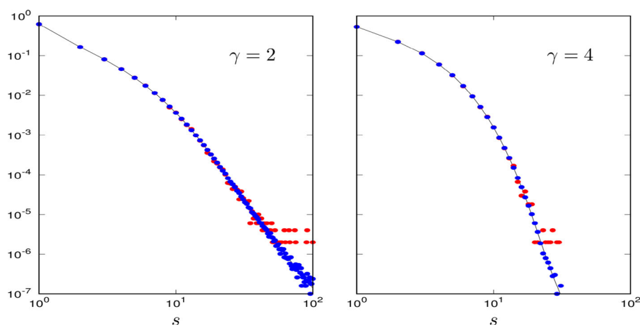
Fig. 3 Empirical estimates of p(s) versus s with data sequences of length t = 10^6 (red) and t = 10^8 (blue) generated by the models defined by c_t = 1/4 + (1/4)(1+t)^{-\gamma} for t \geq 0 with \gamma = 2 (left) and \gamma = 4 (right). Black curves are the theoretical limits p(s) (Color figure online)
