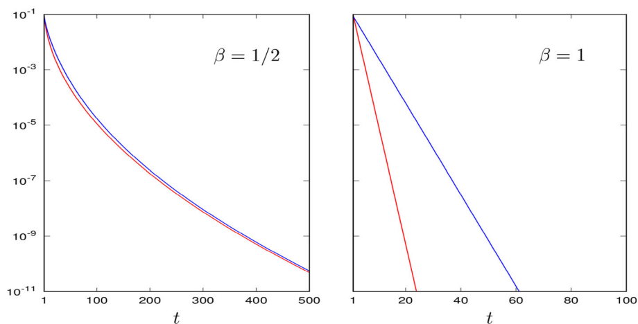
Fig. 2 Autocovariance \rho_t (red) and (1/\mu^3) \sum_{n>t} Q(n) (blue) versus t for the inverse problem with c_t = 1/4 + (1/4)e^{-t^\beta} for t \geq 0 with \beta = 1/2 (left) and \beta = 1 (right) (Color figure online)
