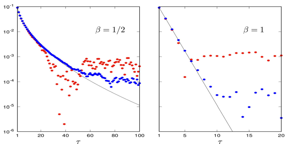
Fig. 6 Empirical estimates of \rho_\tau versus \tau with data sequences of length t = 10^6 (red) and t = 10^8 (blue) generated by the models defined by c_t = 1/4 + (1/4)e^{-t^\beta} for t \geq 0 with \beta = 1/2 (left) and \beta = 1 (right). Black curves are the theoretical limits \rho_\tau (Color figure online)
