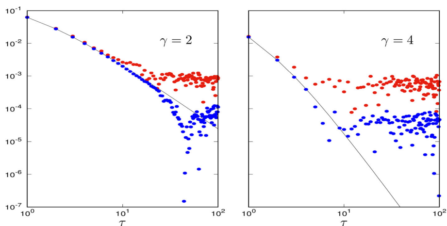
Fig. 5 Empirical estimates of \rho_\tau versus \tau with data sequences of length t = 10^6 (red) and t = 10^8 (blue) generated by the models defined by c_t = 1/4 + (1/4)(1+t)^{-\gamma} for t \geq 0 with \gamma = 2 (left) and \gamma = 4 (right). Black curves are the theoretical limits \rho_\tau (Color figure online)
