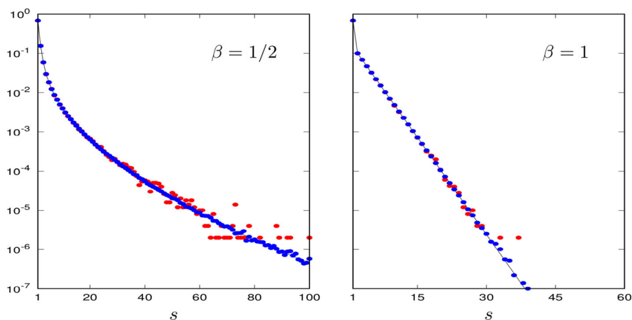
Fig. 4 Empirical estimates of p(s) versus s with data sequences of length t = 10^6 (red) and t = 10^8 (blue) generated by the models defined by c_t = 1/4 + (1/4)e^{-t^\beta} for t \geq 0 with \beta = 1/2 (left) and \beta = 1 (right). Black curves are the theoretical limits p(s) (Color figure online)
