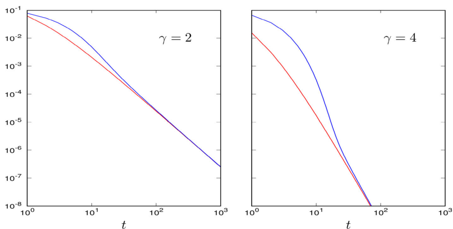
Fig. 1 Autocovariance \rho_t (red) and (1/\mu^3) \sum_{n>t} Q(n) (blue) versus t for the inverse problem with c_t = 1/4 + (1/4)(1+t)^{-\gamma} for t \geq 0 with \gamma = 2 (left) and \gamma = 4 (right) (Color figure online)
