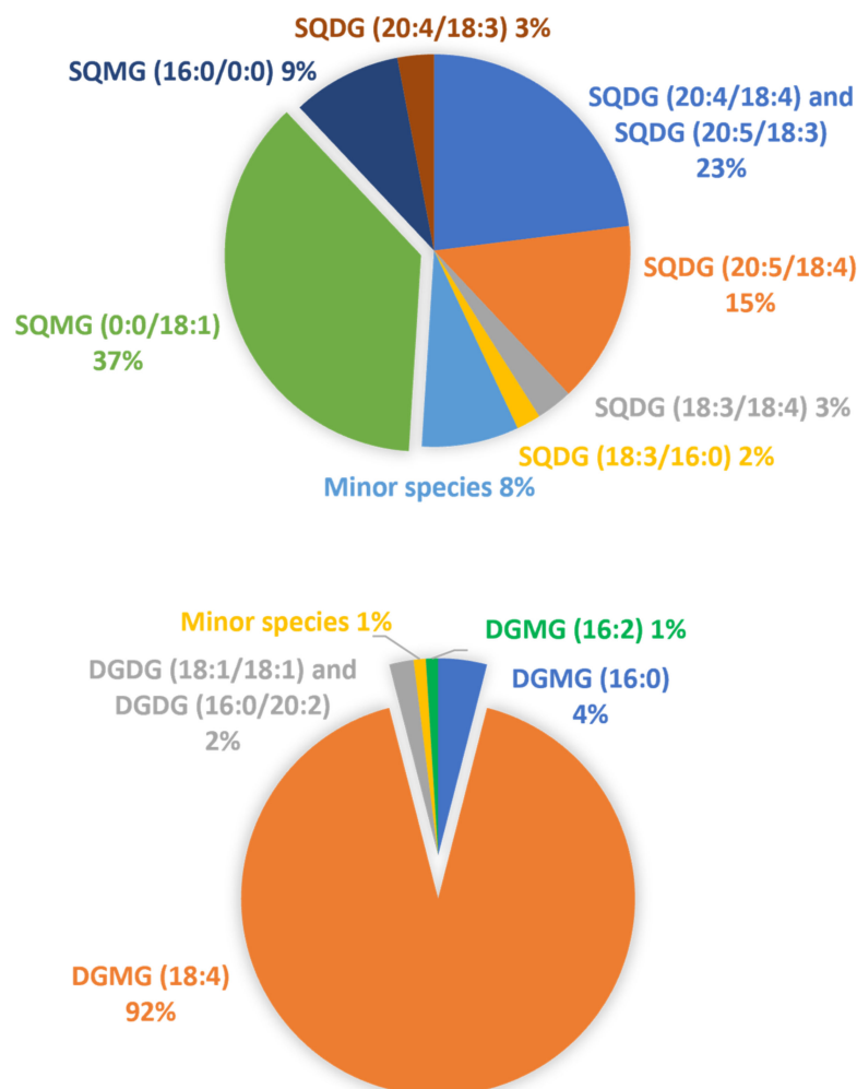
Figure 6. Representation of the relative abundance of the major SQDG (upper panel) and DGDG (lower panel) classes and the relevant lyso-forms (SQMG/DGMG) in the wakame seaweed lipid extracts.
