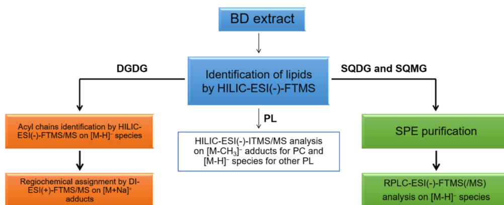
Figure 1. Adopted workflow: lipids from algal samples were extracted by using the procedure described by Bligh and Dyer. HILIC-ESI(-)-FTMS(/MS) and HILIC-ESI(-)-ITMS/MS were employed, in synergy, to characterize PL and DGDG; the regiochemistry of DGDG was assessed using direct infusion (DI)-ESI(+)-FTMS/MS analyses on the corresponding sodium adducts. RPLC-ESI(-)-FTMS/MS, following SPE-based purification, was adopted for the characterization of sulfur-containing glycolipids SQDG and SQMG.
