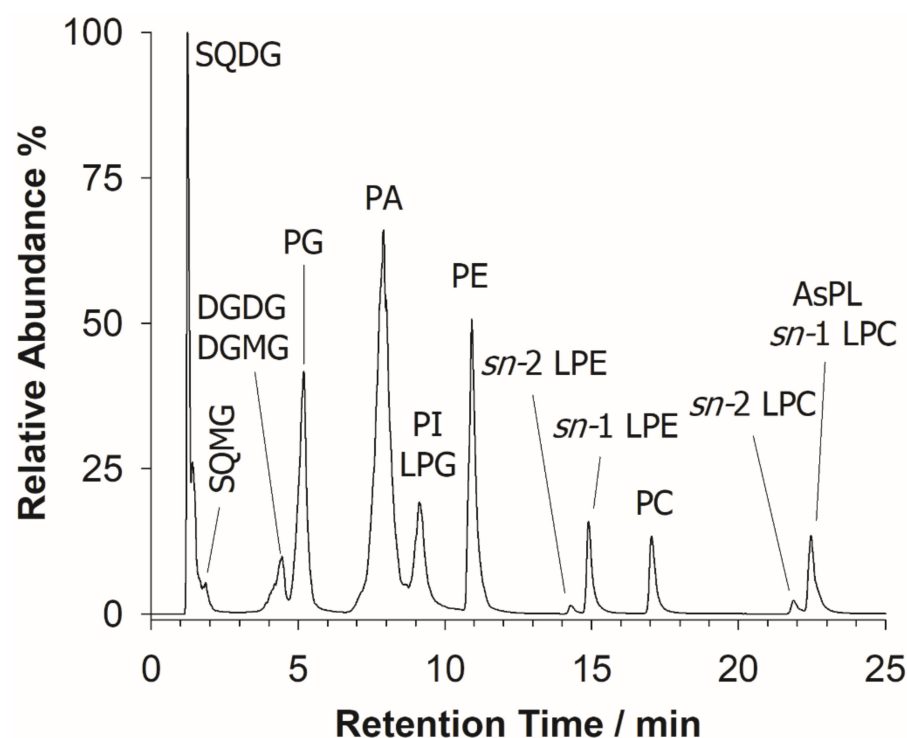
Figure 2. A typical total ion current (TIC) chromatogram arising from the HILIC-ESI(-)-FTMS full scan analysis of the BD extract of wakame seaweed. Sulfoquinovosyl diacylglycerols (SQDG), sulfoquinovosyl monoacylglycerols (SQMG), digalactosyl diacylglycerols (DGDG), digalactosyl monoacylglycerols (DGMG), phosphatidic acids (PA), phosphatidylinositols (PI), phosphatidylglycerols (PG), lyso-PG (LPG), phosphatidylethanolamines (PE), lyso-PE (LPE), phosphatidylcholines (PC), lyso-PC (LPC), and arsenosugar PL (AsPL) are labeled in the figure.
