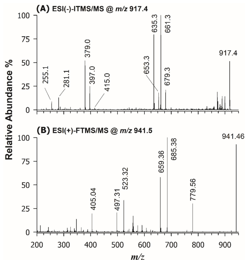
Figure 4. (A) ESI(-)-ITMS/MS spectrum, obtained after HILIC separation of the BD extract of U. pinnatifida , of the [M-H]^- ion detected at m/z 917.4; (B) ESI(+)-FTMS/MS spectrum, obtained upon direct infusion of the same BD extract after sodium acetate addition, for the [M+Na]^+ ion detected at m/z 941.46. The final assignment inferred from the two spectra was DGDG 16:0/18:1.
