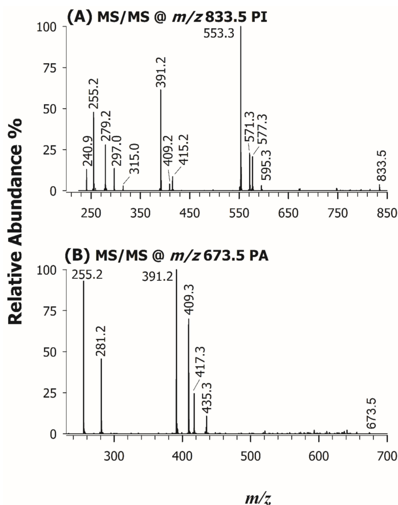
Figure 5. ESI(-)-ITMS/MS spectra of the precursor ions at m/z 833.5 (A) and 673.5 (B), assigned to PI 16:0/18:2 and PA 16:0/18:1, respectively.
