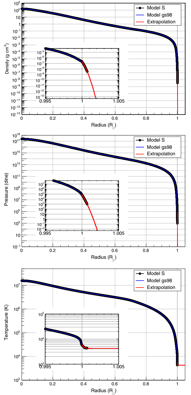
FIG. 2. Density (top panel), pressure (middle panel), and temperature (bottom panel) as a function of the radial distance from the Sun center in units of R_{\odot} . The black dots indicate the model S [28]; the blue line is the model gs98 [27]; the red line is the present extrapolation. The inset shows a zoom near the Sun radius.
