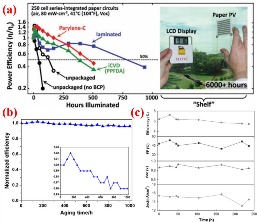
Figure 11. Long term stability of paper solar cells. (a) OPV module encapsulated with plastic lamination (blue), or CVD deposition of Parylene C (red) or PPFCA (green) films. Reproduced with permission. [46] Copyright 2011, John Wiley and Sons. Samples were kept in air at constant illumination (80mW/cm 2 ). (b) Long-term stability of DSSC with a cellulose photoanode at 50°C in dark. Reproduced with permission. [103] Copyright 2017, Elsevier Ltd. All rights reserved. (c) Shelf-life test of PSC on paper. Reproduced with permission. [53] Copyright 2016, Elsevier Ltd. All rights reserved.
