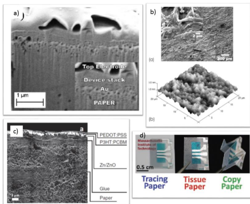
Figure 1. a) Cross section SEM image of a perovskite SC deposited on commercial electronic paper. Reproduced with permission; [31] Copyright 2017, IEEE. b) Top: SEM Micrograph of newspaper before the treatment. Bottom: AFM topography of the same paper after parylene
