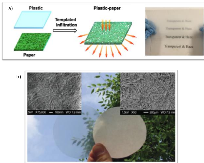
Figure 2 a) Concept of plastic-paper production and a photography of the transparency&haze effect. Reproduced with permission. [21] Copyright 2012, Royal Society of Chemistry. b) Nanopaper (left) and paper (right). Optically transparent paper (left) is composed by 150 nm cellulose nanofibers. The upper left inset, with a scale bar of 100 nm, shows a SEM micrograph of the surface of transparent nanopaper. Conventional cellulose paper (right) is composed by 30 μm pulp fibres. The upper right inset, with a scale bar of 200 μm, shows the SEM micrograph of the surface of a sample of filter paper. Reproduced with permission. [51] Copyright 2009, John Wiley and Sons.
