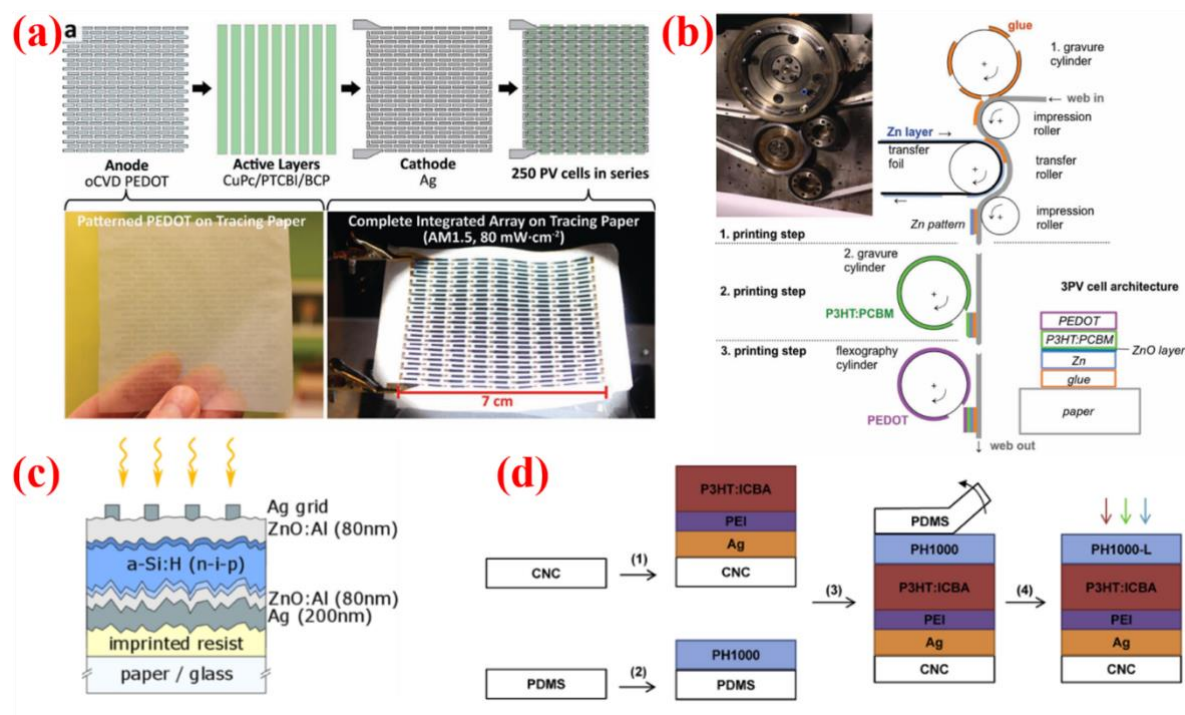
Figure 5 Deposition of bottom electrode (a-d) and lamination of top electrode (e) on cellulose paper using different deposition techniques. (a) Oxidative chemical vapour deposition (oCVD) of PEDOT grid on tracing paper. Organic solar module contained 250 cells. Reproduced with permission. [46] Copyright 2011, John Wiley and Sons. (b) Roll-to-roll (R2R) lamination of Zn electrode on glossy paper, gravure printing of P3HT:PCBM active layer, and flexography of conductive PEDOT top electrode. Reproduced with permission. [9] Copyright 2011, John Wiley and Sons. (c) Paper surface modification with an UV resistive resin. Resin allowed a controllable design of surface pattern which enhanced the light scattering in an a-Si solar cell. Reproduced with permission. [110] Copyright 2017, John Wiley and Sons. (d)
