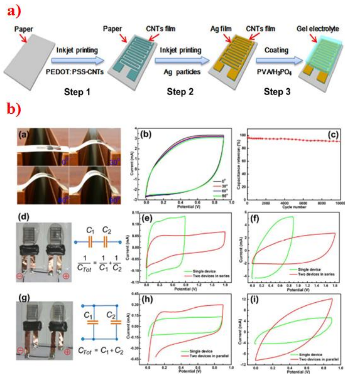
Figure 8: Symmetrical supercapacitor realized via inkjet printing: a) realization process b) electrical performances after bending tests. Reproduced with permission [144] . Copyright 2016, Journal of Materials Chemistry A.
