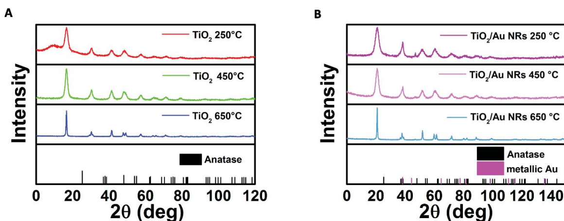
Figure 5. XRD Diffraction patterns of bare \text{TiO}_2 (A) and \text{TiO}_2/\text{AuNRs} samples (B) at different calcinations temperature: 250 °C, 450 °C and 650 °C. Bragg hkl reflections positions for anatase phase (black markers), metallic Au (pink markers).
