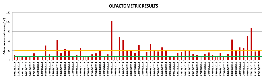
Figure 5. Olfactometric results, expressed in \text{ou}_E/\text{m}^3 , measured during odor events. The bars indicate the maximum odor concentration measured during each odor event. The graph does not report the events for which the results were not considered valid and displays only the maximum odor concentration in cases where two activations happened at different time intervals of the same day.
