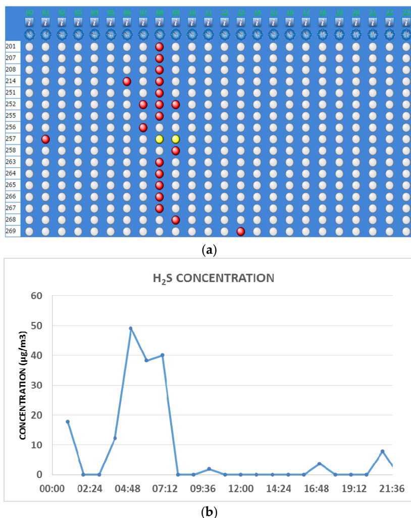
Figure 7. (a) Synoptic hourly visualization of complaints recorded by Odortel® on 1 August 2014 (each row refers to the annoyed receptor and each column indicates each hour of the day); (b) Analytical responses of \text{H}_2\text{S} concentrations, recorded on 1 August 2014.
