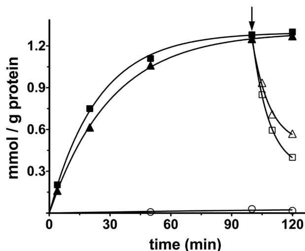
FIGURE 7. Time course of reconstituted [^{14}\text{C}]\text{ADP}/\text{CoA} and [^{14}\text{C}]\text{ADP}/\text{dephospho-CoA} exchanges and efflux of [^{14}\text{C}]\text{ADP} from proteoliposomes after addition of unlabeled CoA or dephospho-CoA. 40 \mu\text{M} [^{14}\text{C}]\text{ADP} was added to liposomes reconstituted with SLC25A42 and preloaded internally with 2 mM CoA or dephospho-CoA (exchange, \blacktriangle and \blacksquare , respectively) or 2 mM NaCl and no substrate (uniport, \circ ). The arrow indicates the addition of 2 mM nonradioactive CoA ( \triangle ) or dephospho-CoA ( \square ). Similar results were obtained in three independent experiments.
