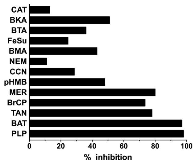
FIGURE 5. Effect of inhibitors on the [ ^{14} C]ADP/ADP exchange by SLC25A42. Proteoliposomes were preloaded internally with 10 mM ADP, and transport was initiated by adding 40 \mu M [ ^{14} C]ADP to liposomes reconstituted with SLC25A42. The incubation time was 2 min. Thiol reagents and \alpha -cyanocinnamate were added 2 min before the labeled substrate. The final concentrations of the inhibitors were 10 \mu M (CAT, carboxyatractylolide; BKA, bongkreic acid), 20 mM (PLP, pyridoxal-5'-phosphate; BAT, bathophenanthroline), 0.2 mM (pHMB, p -hydroxymercuribenzoate; MER, mersalyl), 1 mM (NEM, N -ethylmaleimide; CCN, \alpha -cyanocinnamate), 2 mM (BMA, butylmalonate; FeSu, phenylsuccinate; BTA, 1,2,3-benzenetricarboxylate), 0.1% (TAN, tannic acid), and 0.1 mM (BrCP, bromocresol purple). The values are expressed as a percentage of the [ ^{14} C]ADP/ADP exchange activity, which was 98 \mu mol/min \times g of protein. Similar results were obtained in at least three independent experiments.
