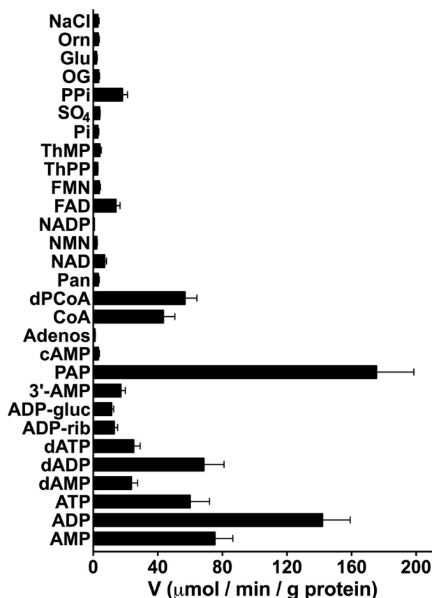
FIGURE 4. Substrate specificity of SLC25A42. Liposomes reconstituted with SLC25A42 were preloaded internally with various substrates (concentration, 10 mM). Transport was started by addition of 60 \mu M [ ^{14} C]ADP and terminated after 2 min. Values are means \pm S.D. of at least three independent experiments. ADP-rib, ADP-ribose; ADP-gluc, ADP-glucose; PAP, adenosine 3',5'-diphosphate; Adenos, adenosine; CoA, coenzyme A; dPCoA, dephospho-CoA; Pan, pantothenate; ThPP, thiamine pyrophosphate; ThMP, thiamine monophosphate; PPi, pyrophosphate; OG, oxoglutarate; Glu, glutamate; Orn, ornithine.
