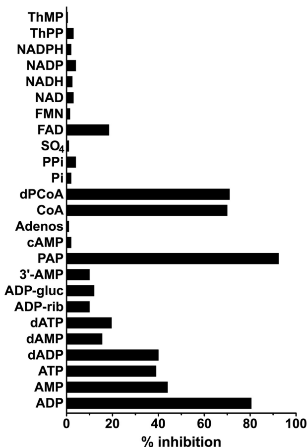
FIGURE 6. Inhibition of the rate of [^{14}\text{C}]\text{ADP}/\text{ADP} exchange by external substrates. Liposomes reconstituted with SLC25A42 were preloaded internally with 10 mM ADP. Transport was started by adding 40 \mu\text{M} [^{14}\text{C}]\text{ADP} and stopped after 2 min. External substrates (concentration, 0.4 mM) were added together with [^{14}\text{C}]\text{ADP} . The values are expressed as a percentage of the [^{14}\text{C}]\text{ADP}/\text{ADP} exchange activity, which was 111 \mu\text{mol}/\text{min} \times \text{g} of protein. Similar results were obtained in at least three independent experiments. ADP-rib, ADP-ribose; ADP-gluc, ADP-glucose; PAP, adenosine 3',5'-diphosphate; Adenos, adenosine; CoA, coenzyme A; dPCoA, dephospho-CoA; PPI, pyrophosphate; ThPP, thiamine pyrophosphate; and ThMP, thiamine monophosphate.
