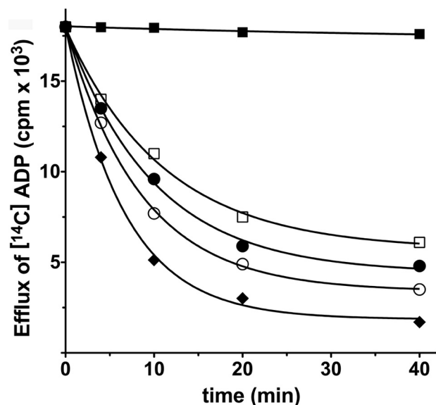
FIGURE 8. Efflux of [^{14}\text{C}]\text{ADP} from proteoliposomes reconstituted in the presence of 2 mM ADP. The internal substrate pool was labeled with [^{14}\text{C}]\text{ADP} by carrier-mediated exchange equilibration. Then the proteoliposomes were passed through Sephadex G-75. The efflux of [^{14}\text{C}]\text{ADP} was started by adding buffer A alone ( \blacksquare ), 0.5 mM PAP in buffer A ( \blacklozenge ), 0.5 mM ADP in buffer A ( \circ ), 0.5 mM CoA in buffer A ( \square ), or 0.5 mM dephospho-CoA in buffer A ( \bullet ). Similar results were obtained in three independent experiments.
